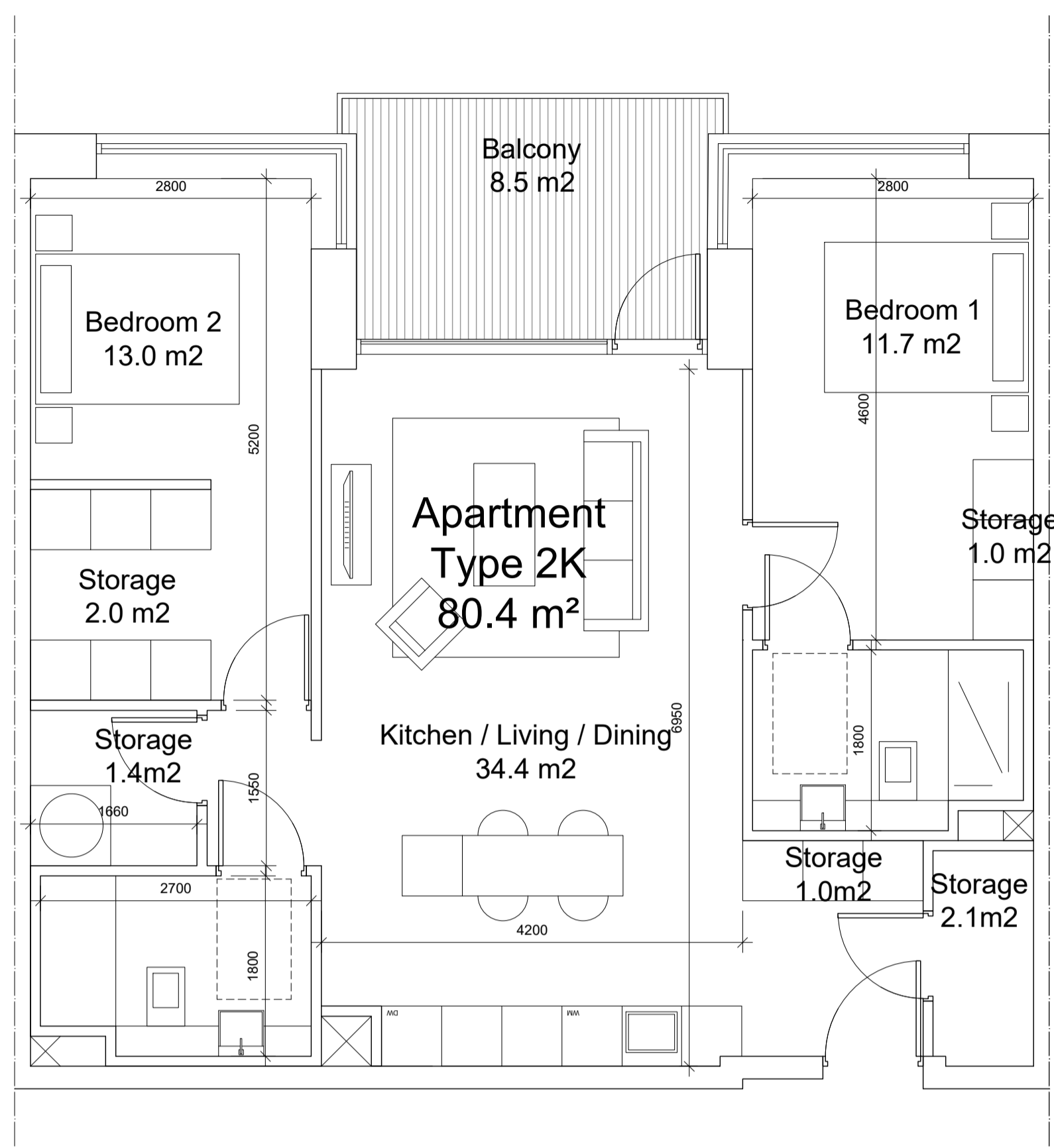
02 2 Bed Apartment - Type 2K (16 Units) SCALE 1:50
