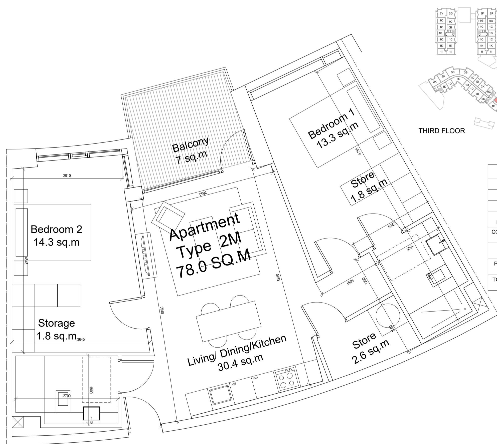
03 2 Bed Apartment - Type 2M (12 units) SCALE 1:50
