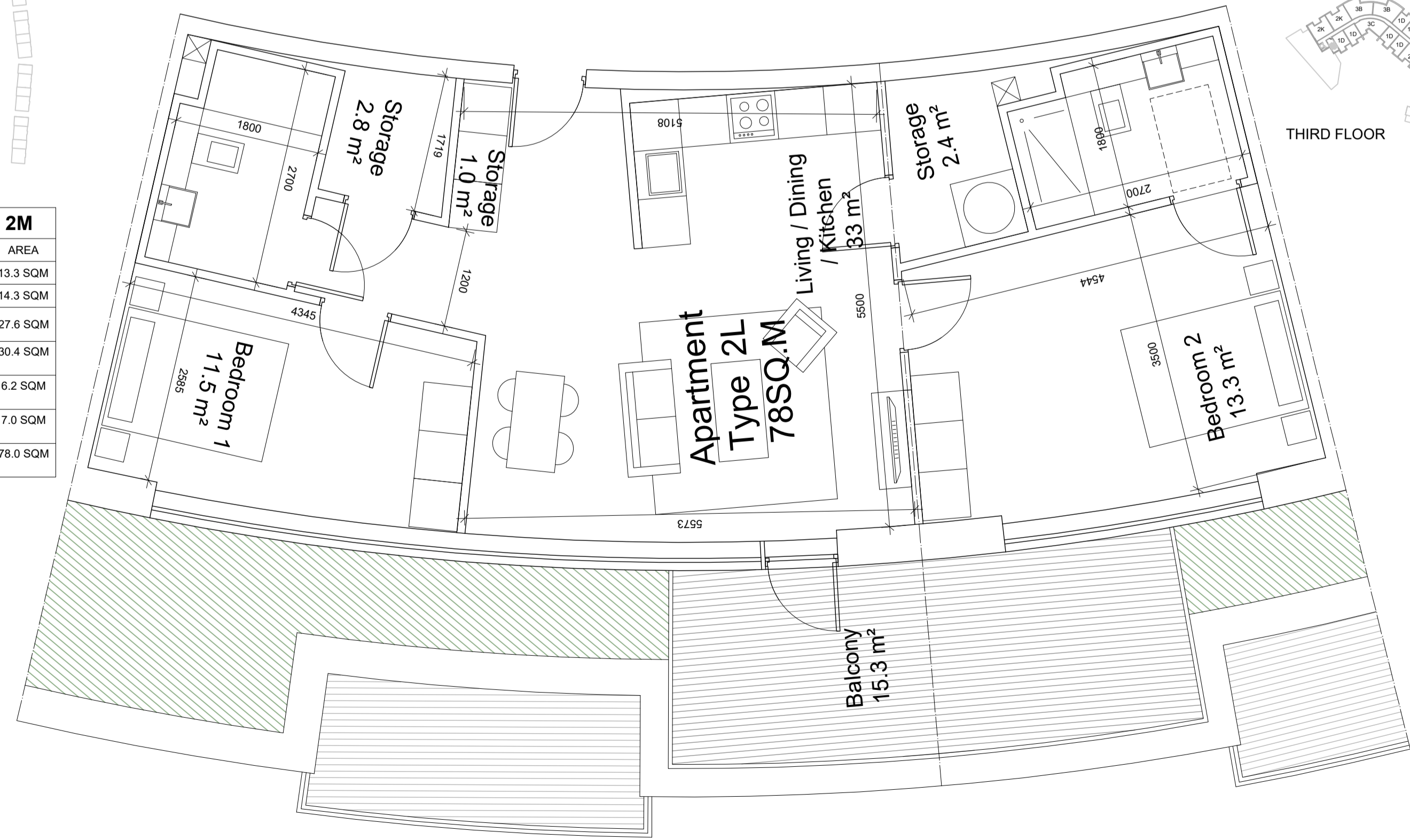
04 2 Bed Apartment - Type 2L (4 units) SCALE 1:50
