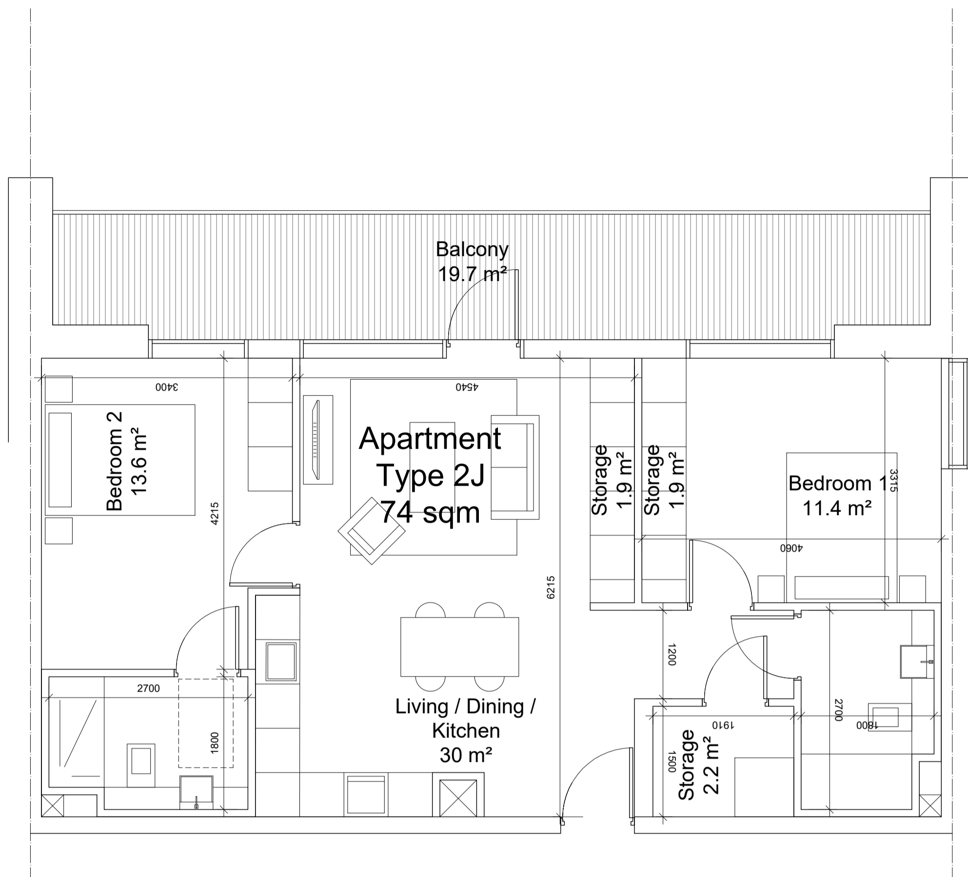
01 2 Bed Apartment - Type 2J (6 units) SCALE 1:50
